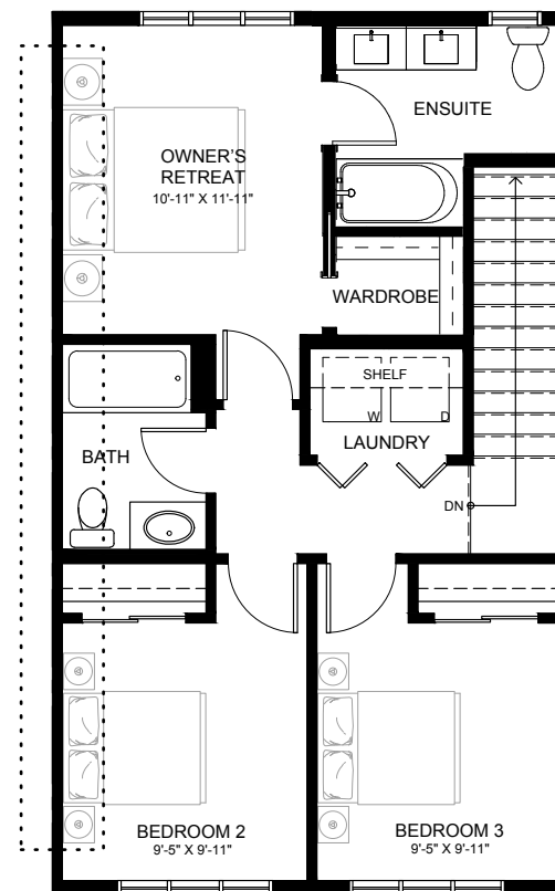
UPPER LEVEL ±680 SQ. FT.
