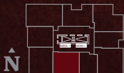
Levels 4 – 34
