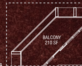
Level 34
