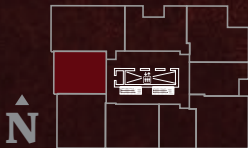
Levels 4 – 34
