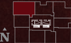
Levels 4 – 34
