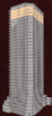
Levels 32 - 34
