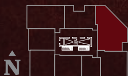
Levels 32 - 34
