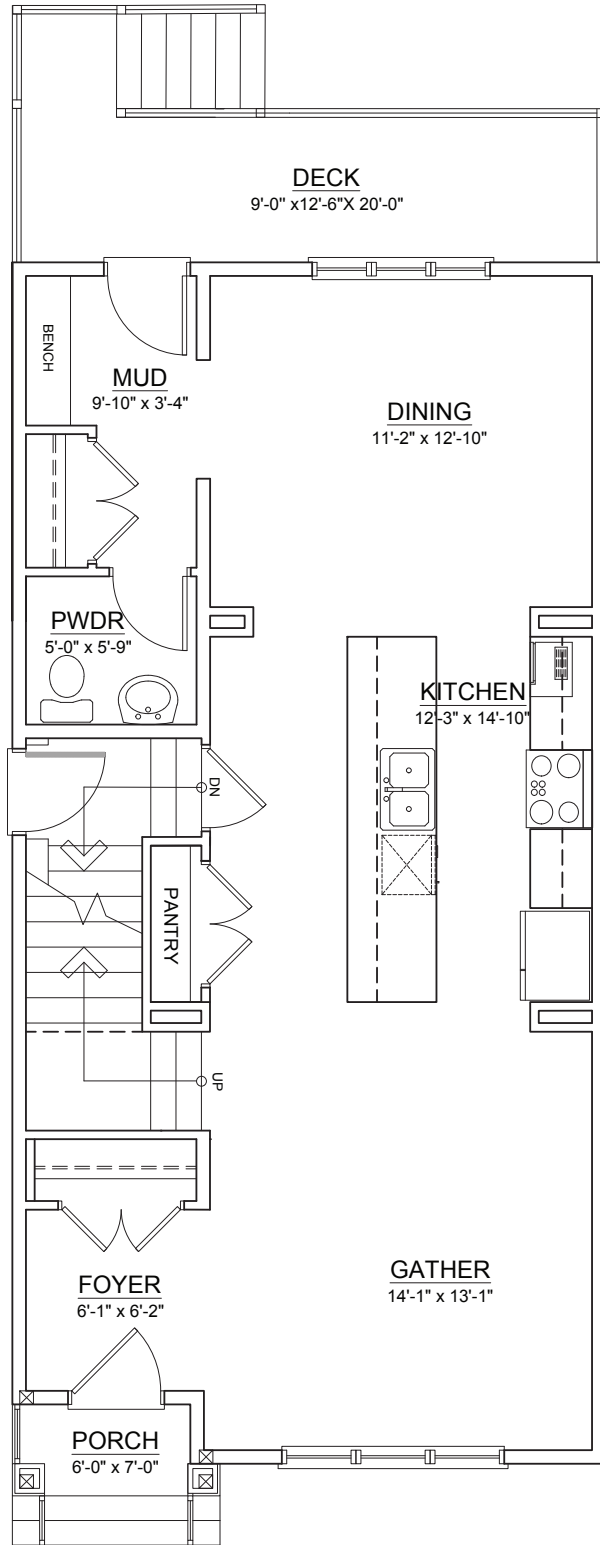
MAIN FLOOR ±798 SQ. FT.
