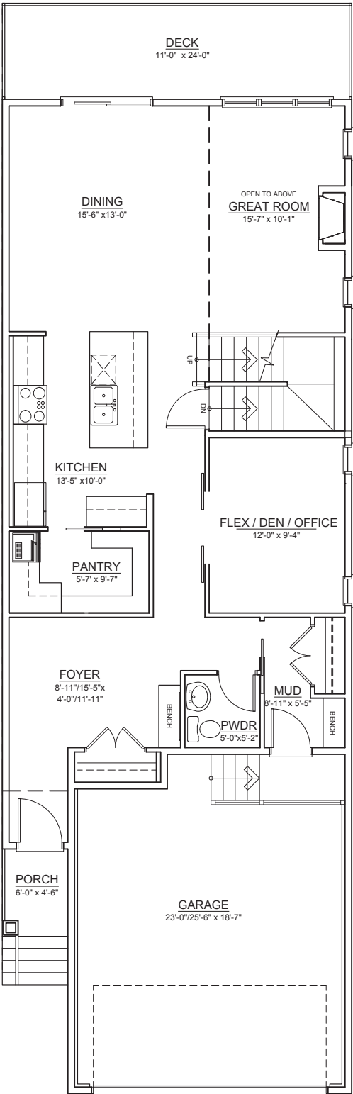
MAIN FLOOR ±1,134 SQ. FT.
