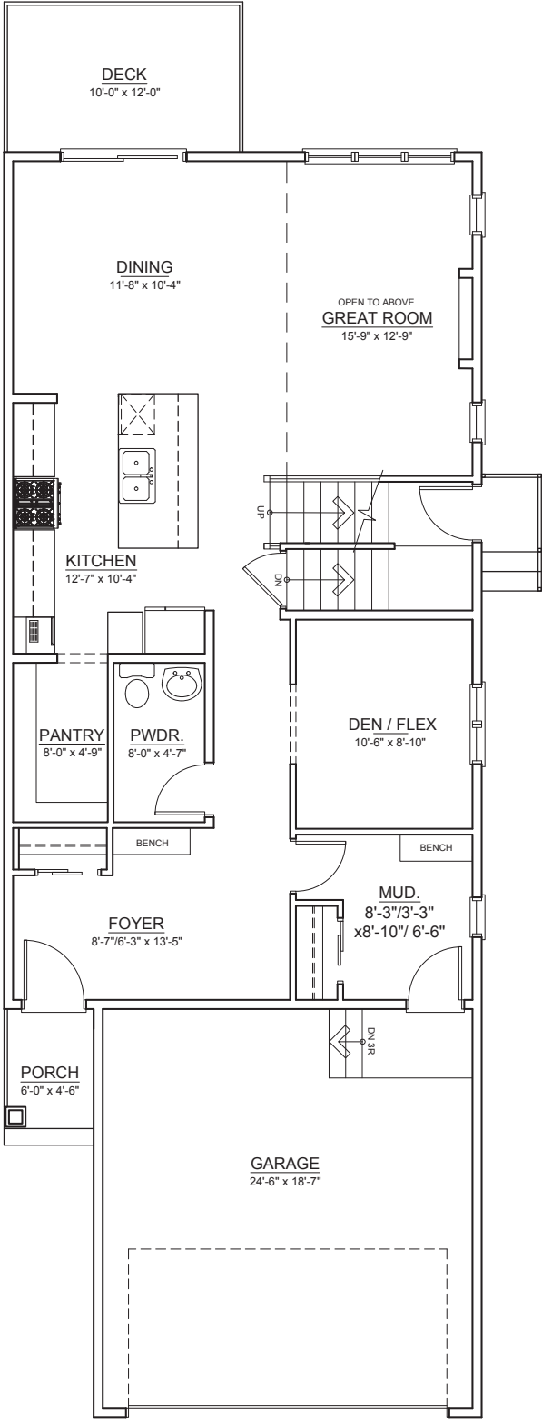
MAIN FLOOR ±1,032 SQ. FT.
