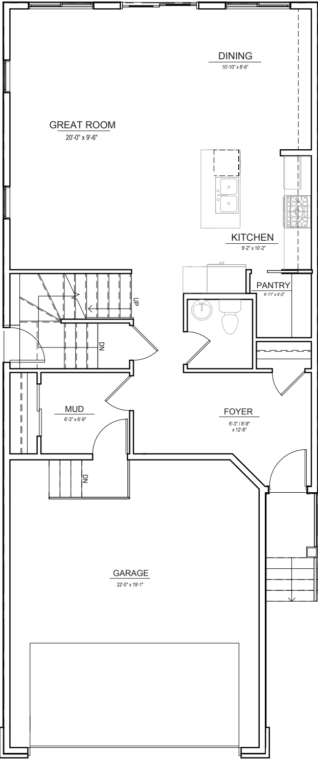
MAIN FLOOR ±855 SQ. FT.
