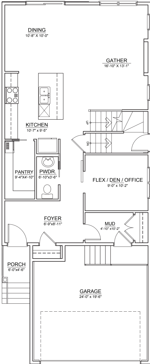
MAIN FLOOR ±957 SQ. FT.
