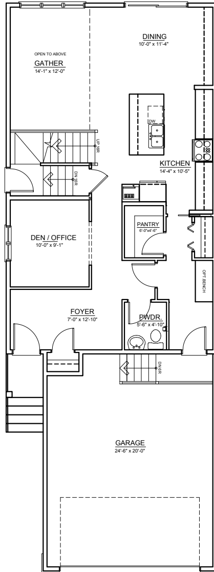
MAIN FLOOR ±900 SQ.FT.
