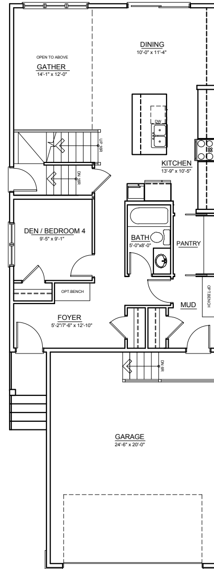
MAIN FLOOR OPTION 3 ± 990 SQ.FT.
