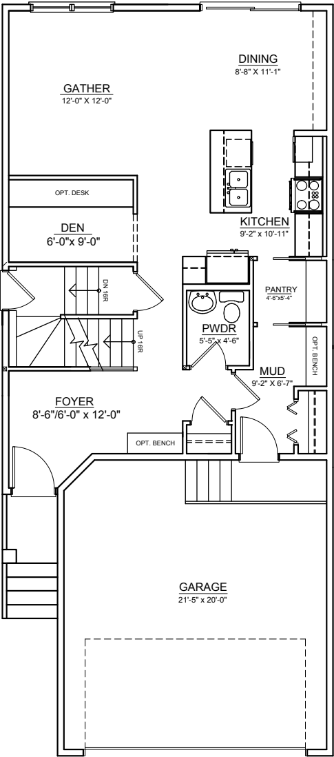
MAIN FLOOR OPTION 2 ±807 SQ.FT.
