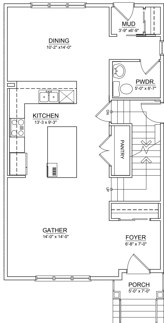
MAIN FLOOR OPTION 2 ± 824 SQ.FT.
