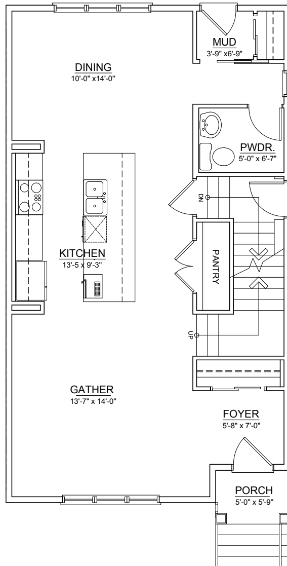
MAIN FLOOR ±824 SQ.FT.
