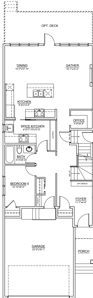
MAIN FLOOR ±1,085 SQ.FT.
