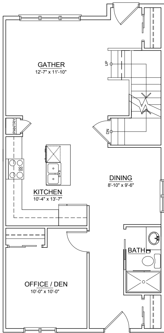
MAIN FLOOR OPTION 2 ±790 SQ.FT.
