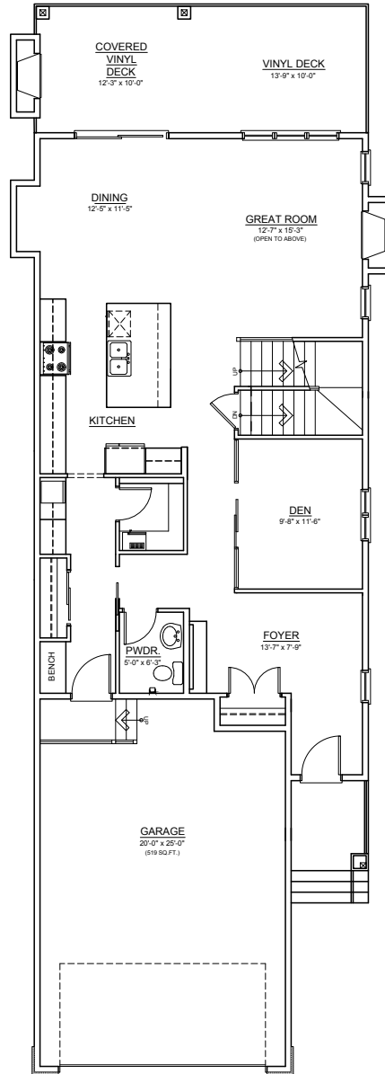
MAIN FLOOR ±1,219 SQ.FT.
