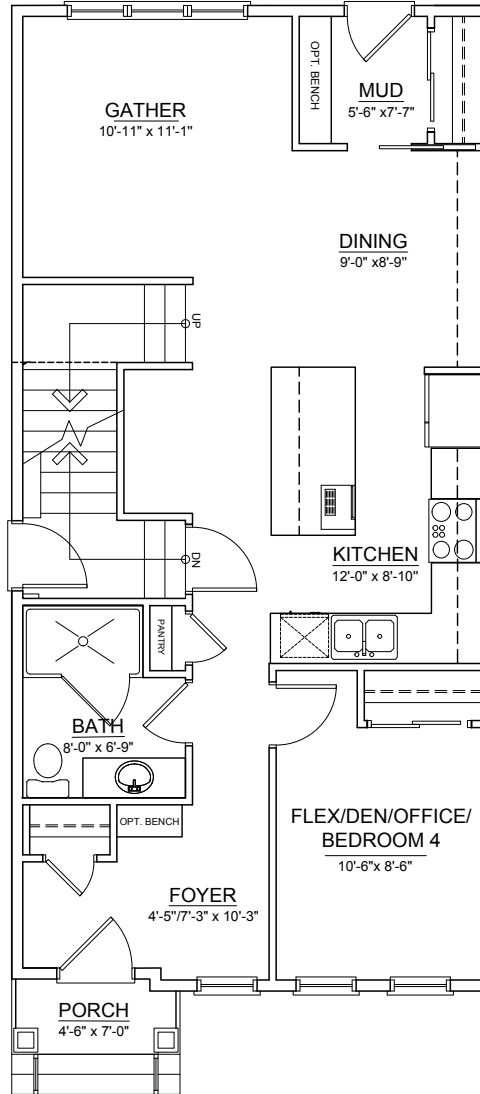
MAIN FLOOR OPTION 3 ±817 SQ.FT.
