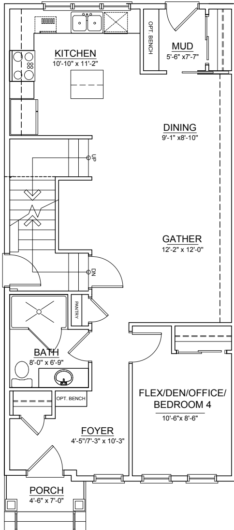
MAIN FLOOR OPTION 2 ±817 SQ.FT.
