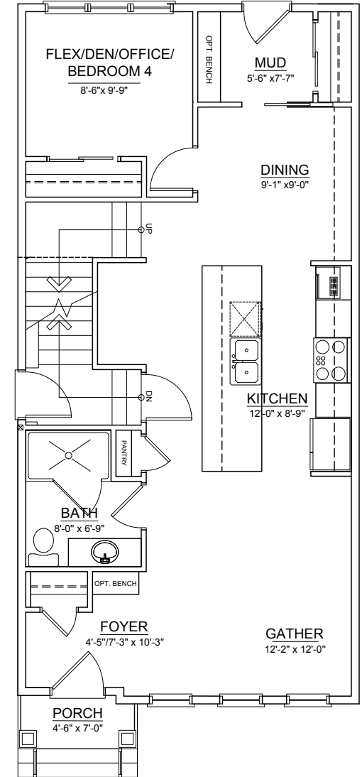
MAIN FLOOR OPTION 4 ±817 SQ.FT.
