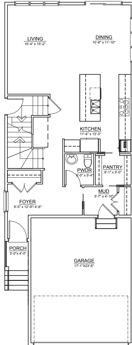
MAIN FLOOR ±826 SQ.FT.
