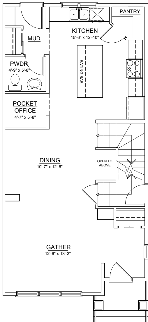
MAIN FLOOR ±788 SQ.FT.
