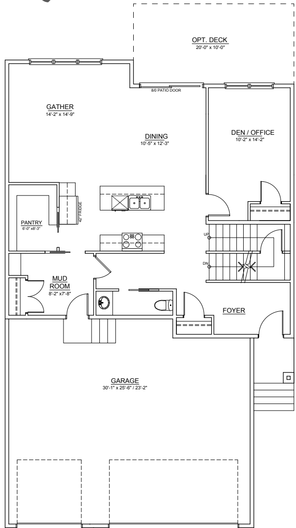
MAIN FLOOR ±1,148 SQ.FT.
