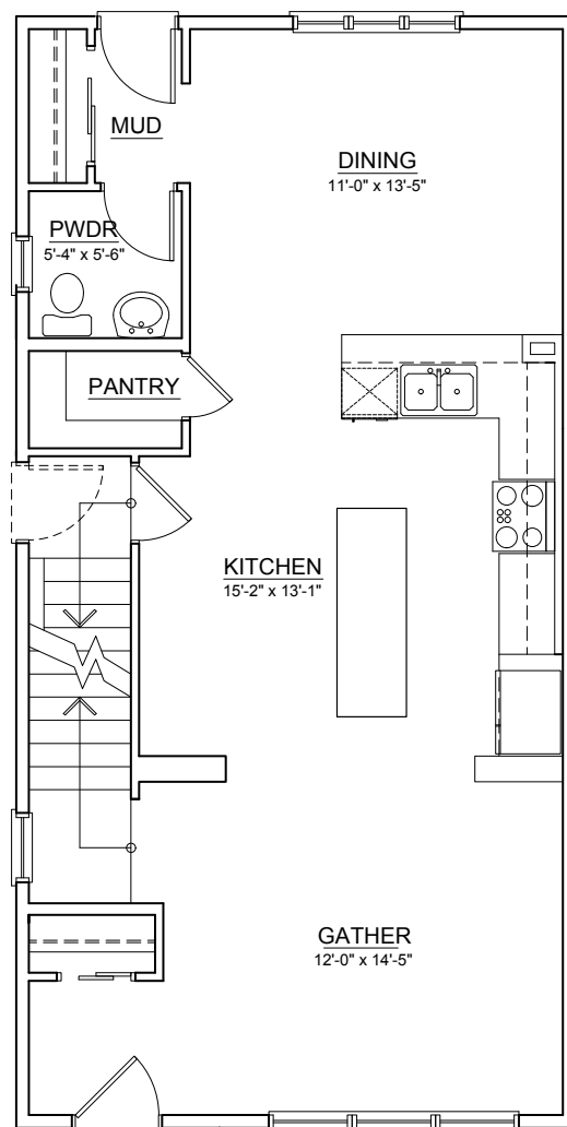
MAIN FLOOR ±800 SQ.FT.
