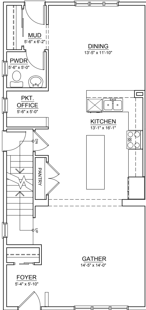
MAIN FLOOR ±857 SQ.FT.
