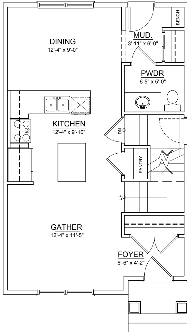
MAIN FLOOR OPTION 2 ±620 SQ.FT.
