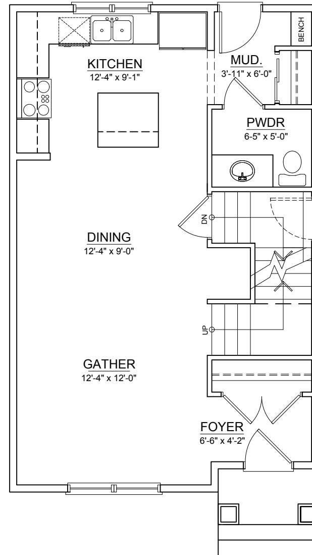
MAIN FLOOR OPTION 3 ±620 SQ.FT.
