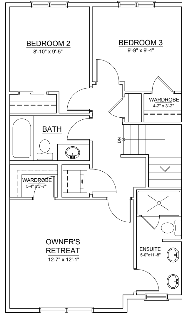
UPPER FLOOR ±680 SQ.FT.
