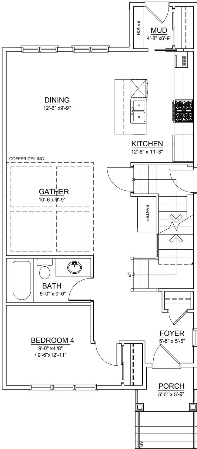
MAIN FLOOR ±871 SQ.FT.
