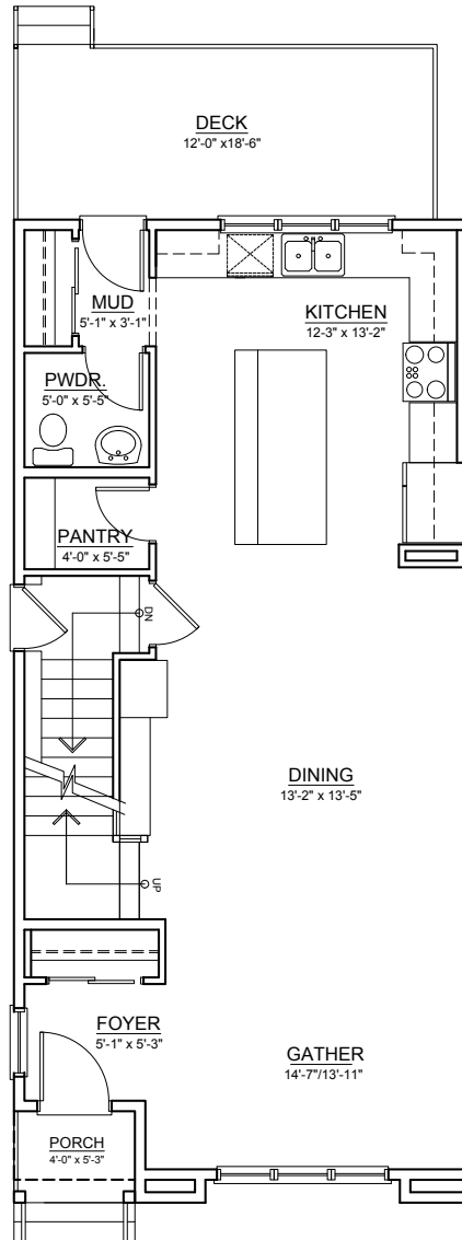
MAIN FLOOR ±830 SQ. FT.
