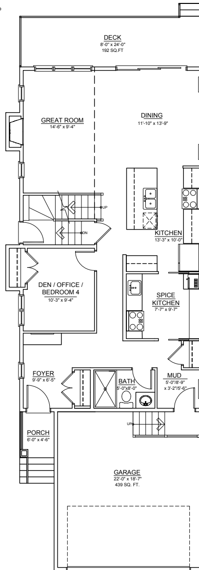
MAIN FLOOR ±1,051 SQ.FT.
