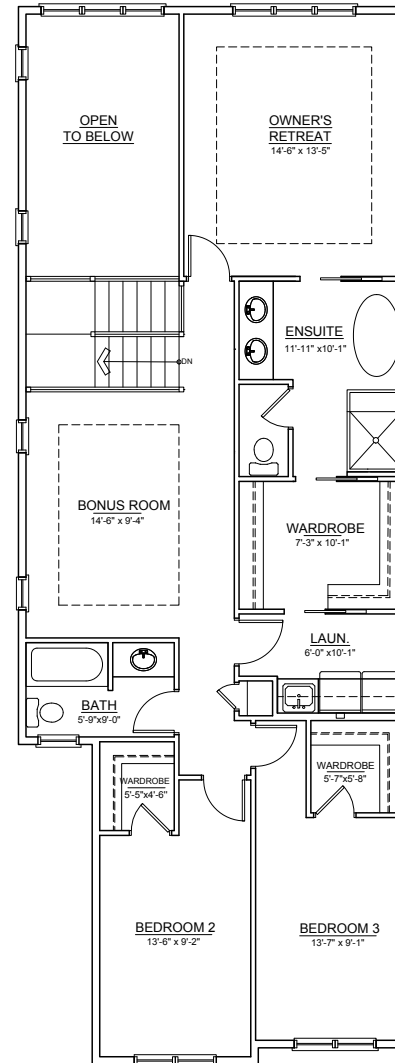
UPPER FLOOR ±1,253 SQ.FT.
