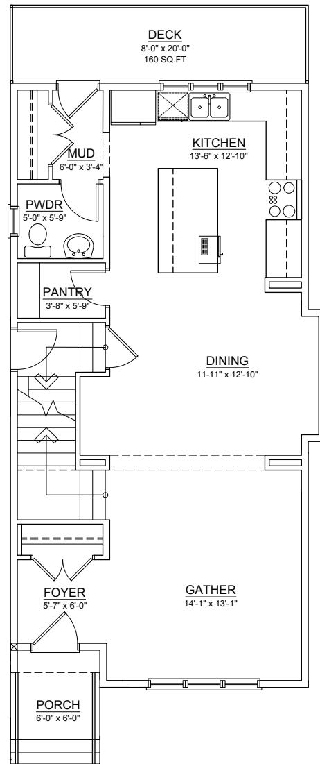
MAIN FLOOR ±804 SQ.FT.
