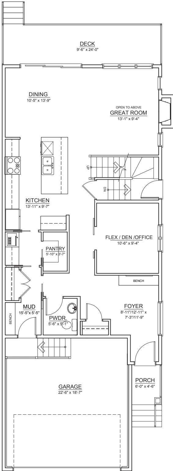
MAIN FLOOR ±1,013 SQ. FT.
