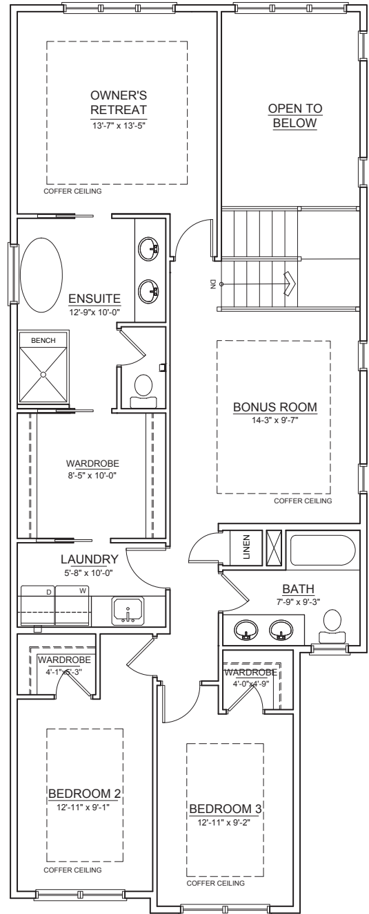
UPPER FLOOR ±1,243 SQ. FT.
