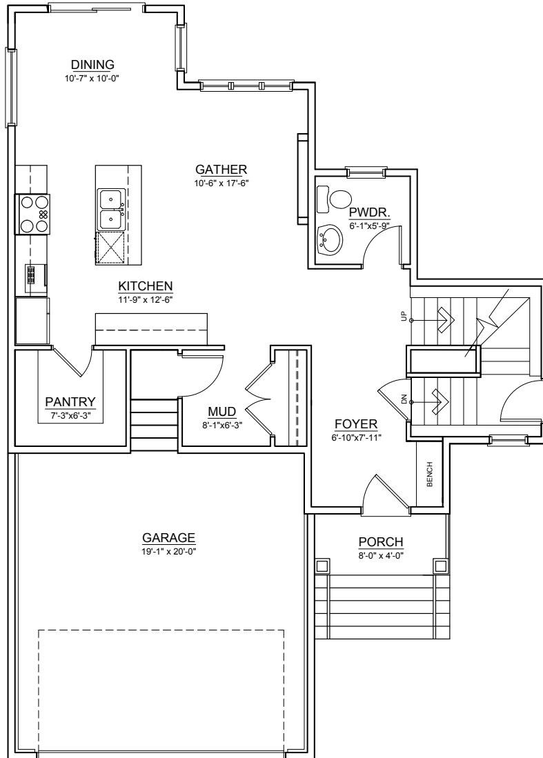
MAIN FLOOR \pm 787 SQ.FT.
