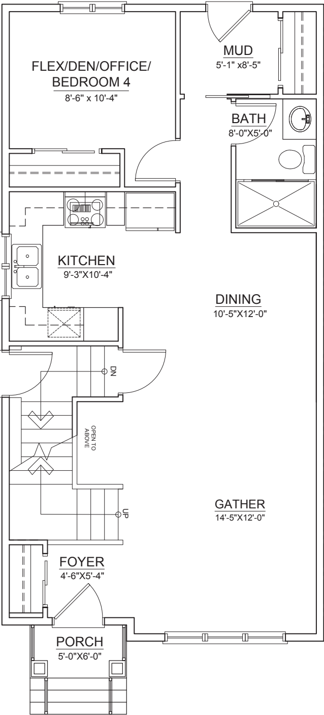
MAIN FLOOR ±776 SQ. FT.
