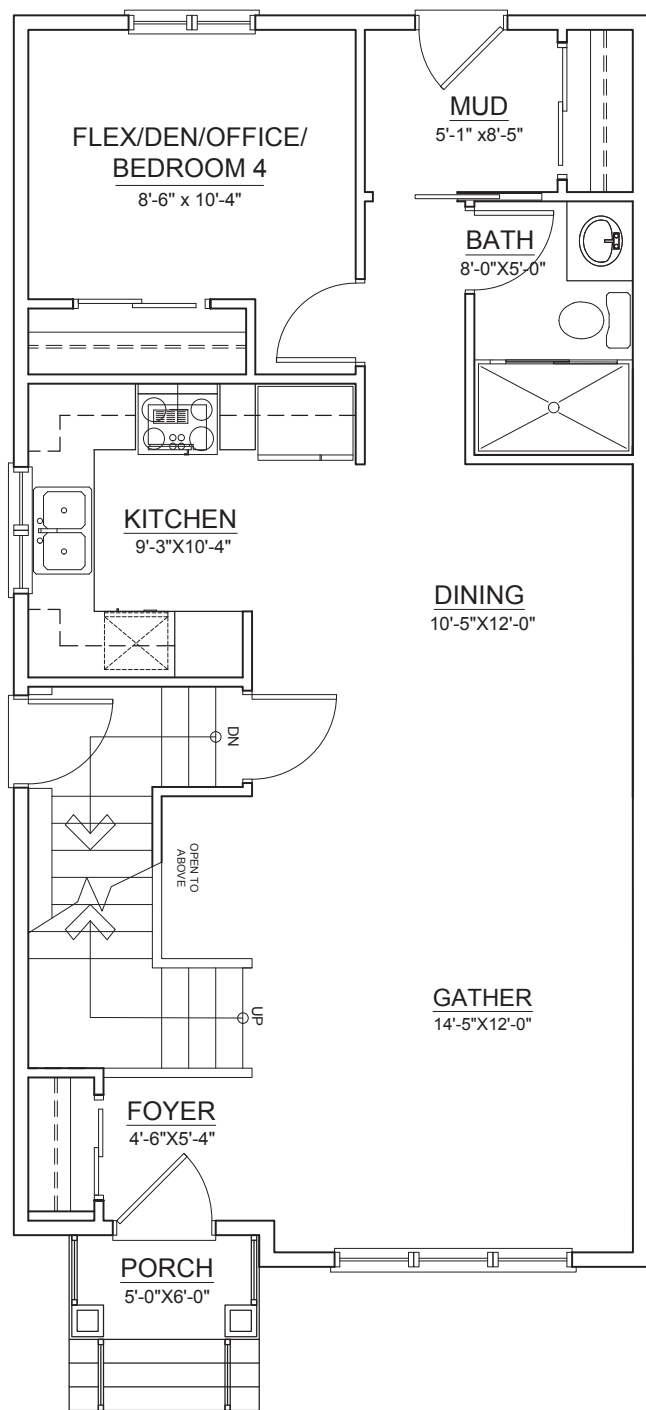
MAIN FLOOR ±778 SQ. FT.
