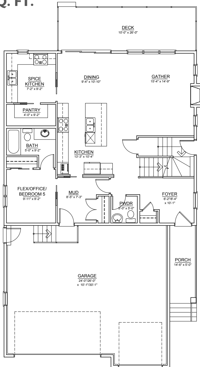
MAIN FLOOR ±1,175 SQ.FT.
