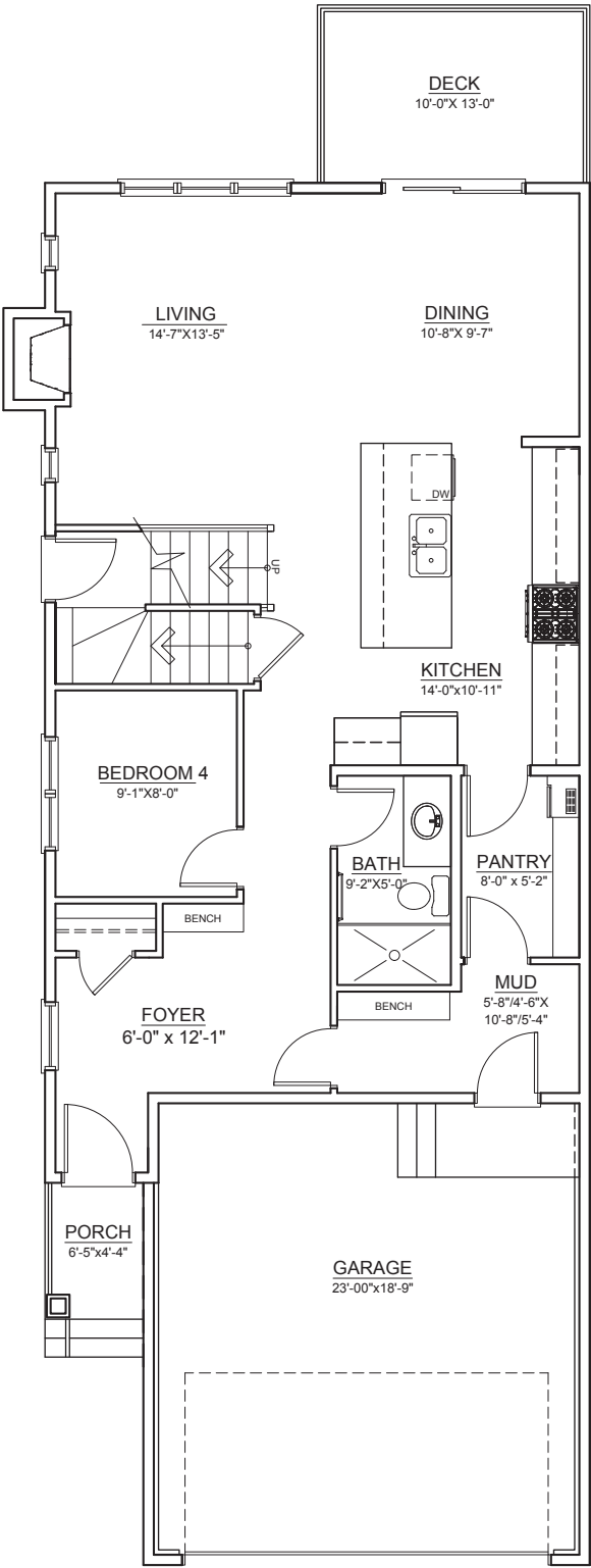
MAIN FLOOR ±997 SQ. FT.
