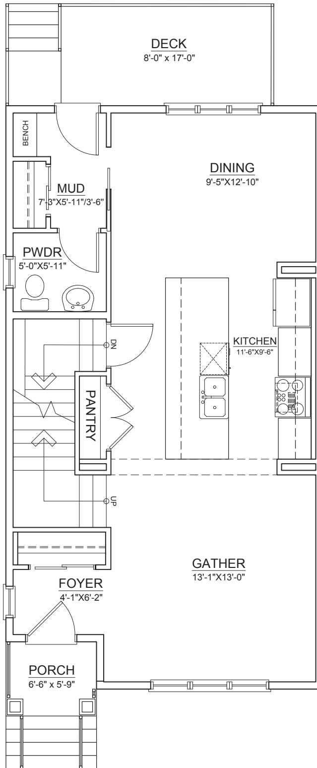
MAIN FLOOR ±723 SQ. FT.
