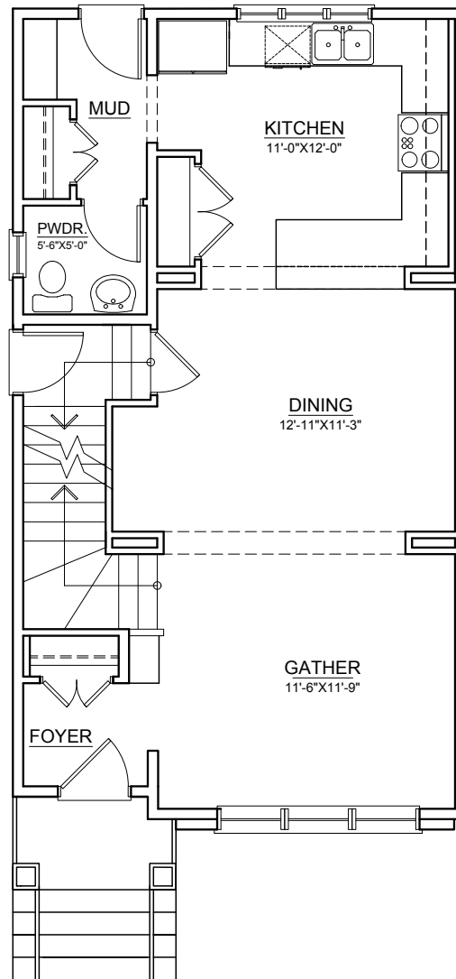
MAIN FLOOR ±714 SQ.FT.
