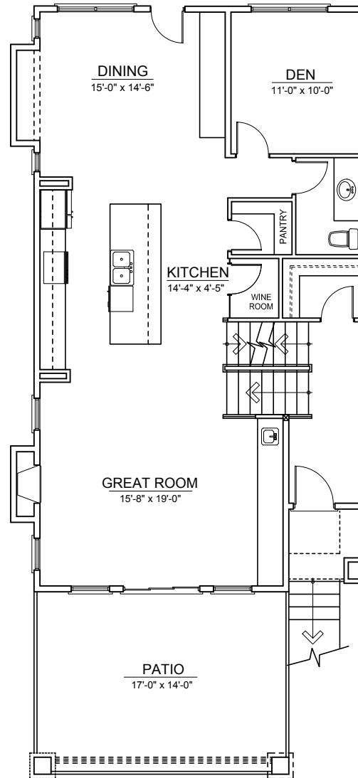
MAIN FLOOR ±1,172 SQ. FT.
