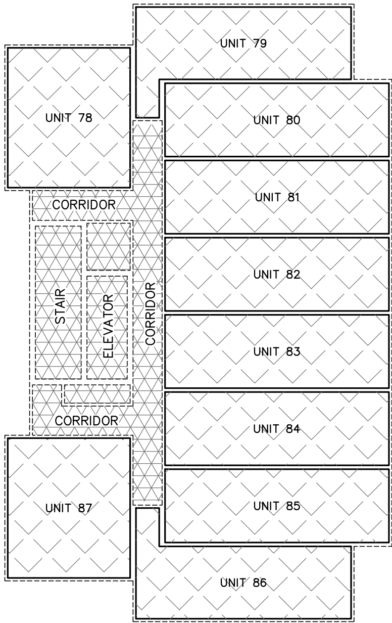
FLOOR 6 SCALE = 1 : 200
