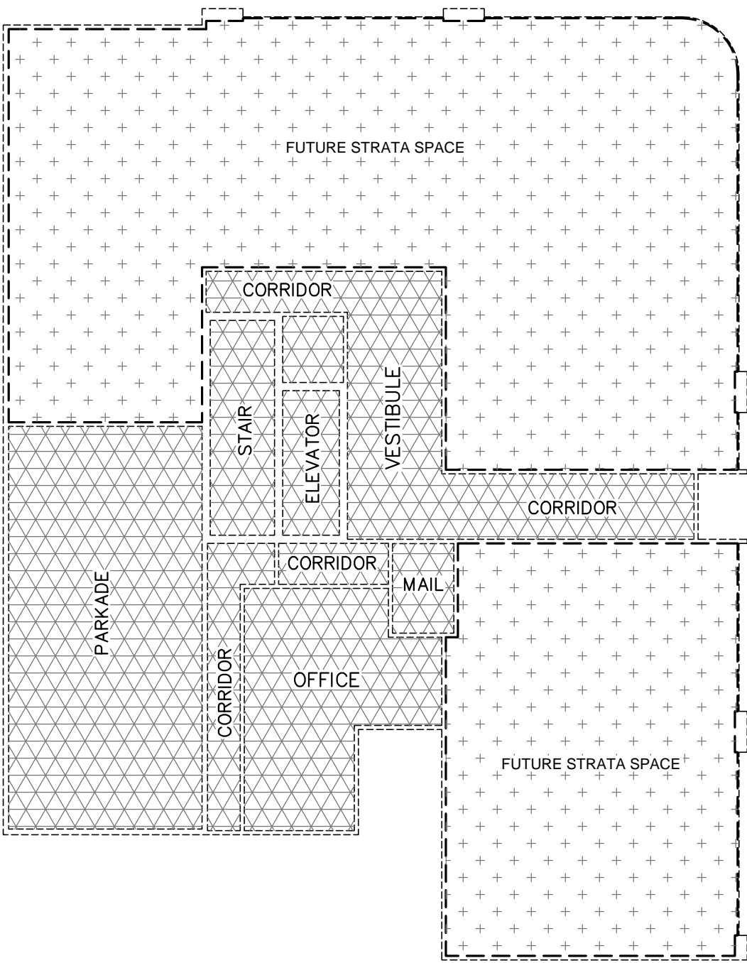
FLOOR 1 SCALE = 1 : 200
