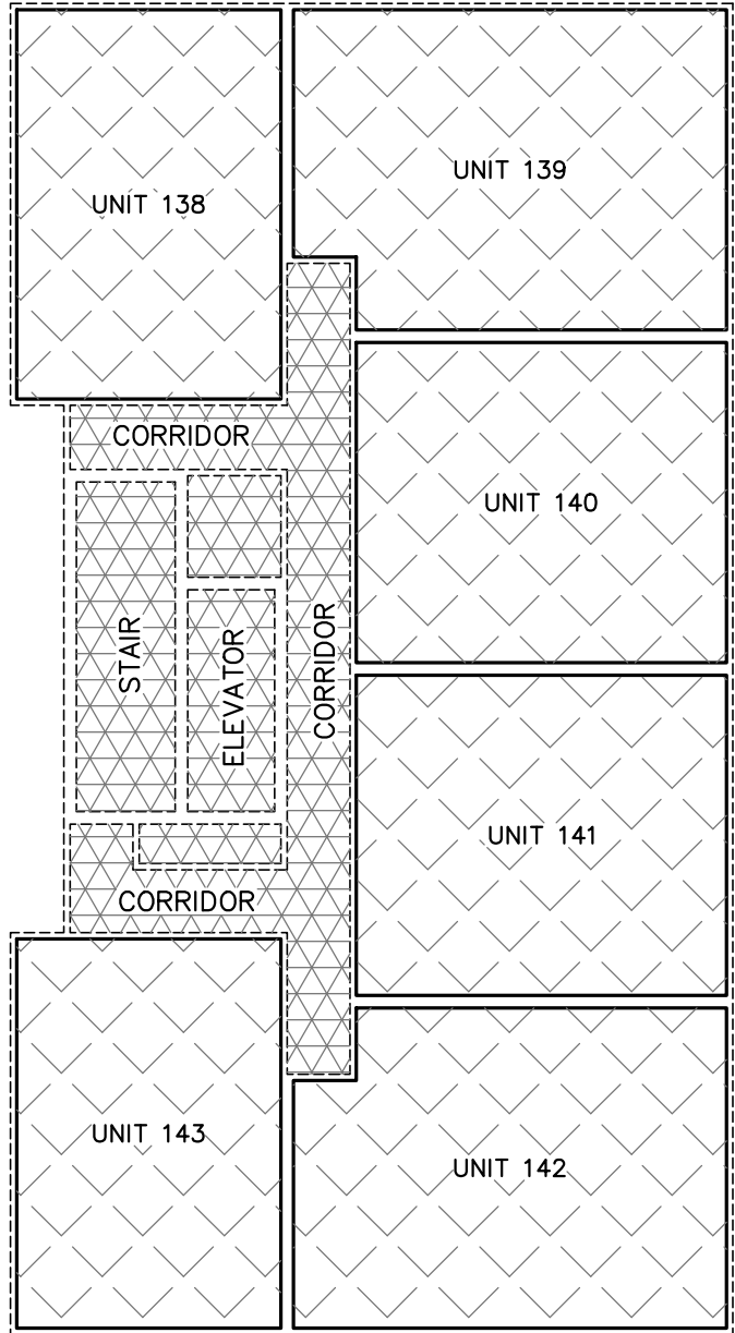
FLOOR 14 SCALE = 1 : 200
