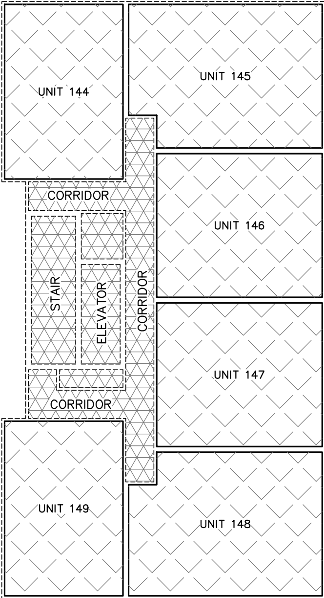
FLOOR 15 SCALE = 1 : 200
