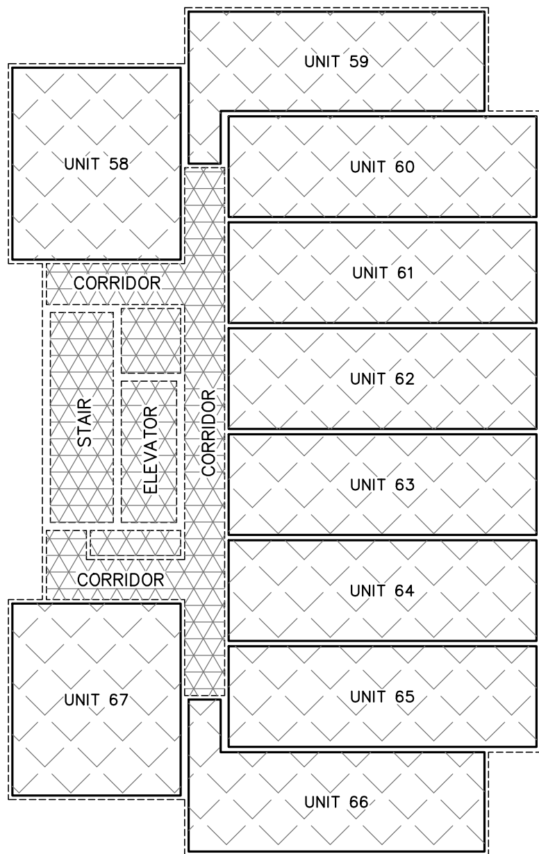
FLOOR 4 SCALE = 1 : 200
