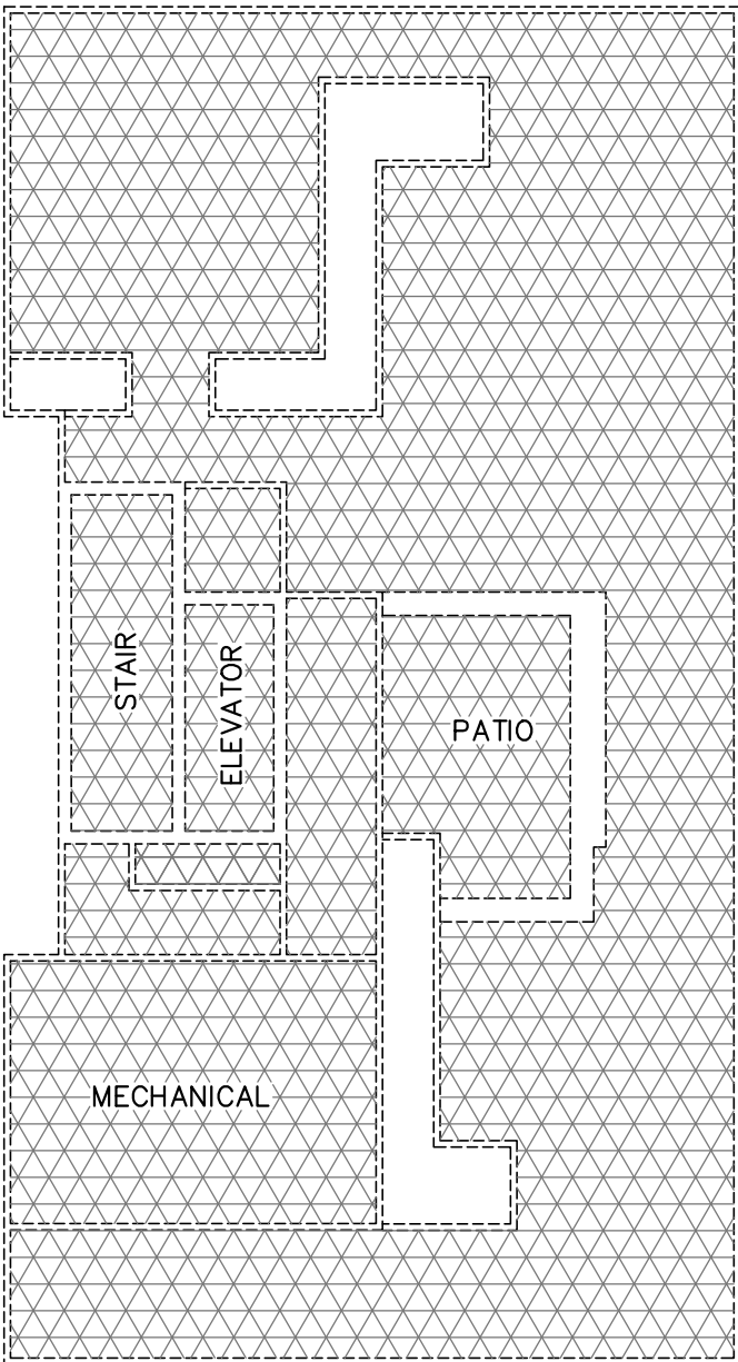
ROOF SCALE = 1 : 200
