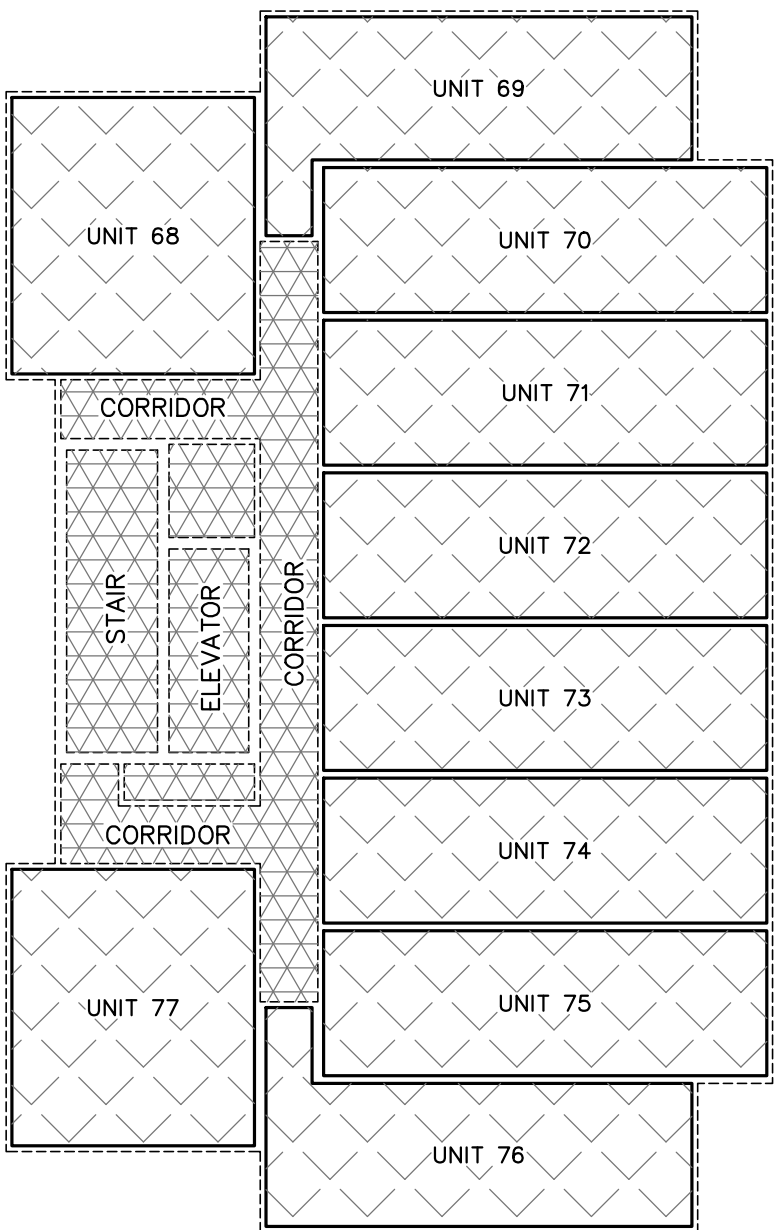
FLOOR 5 SCALE = 1 : 200
