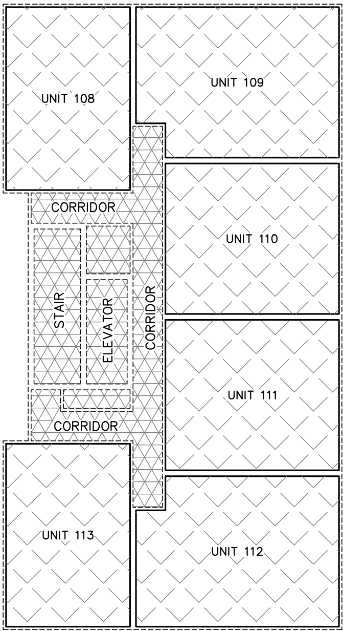
FLOOR 9 SCALE = 1 : 200
