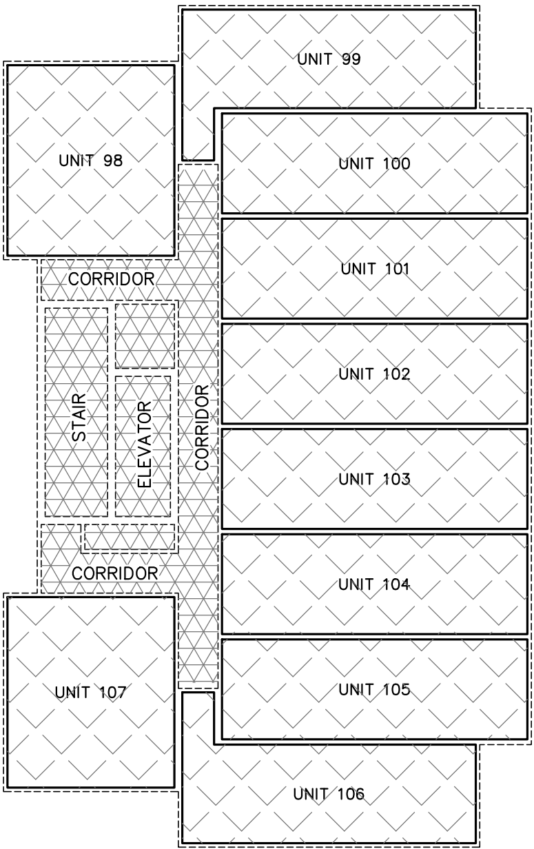
FLOOR 8 SCALE = 1 : 200
