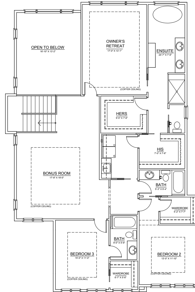
UPPER FLOOR ±1,955 SQ. FT.
