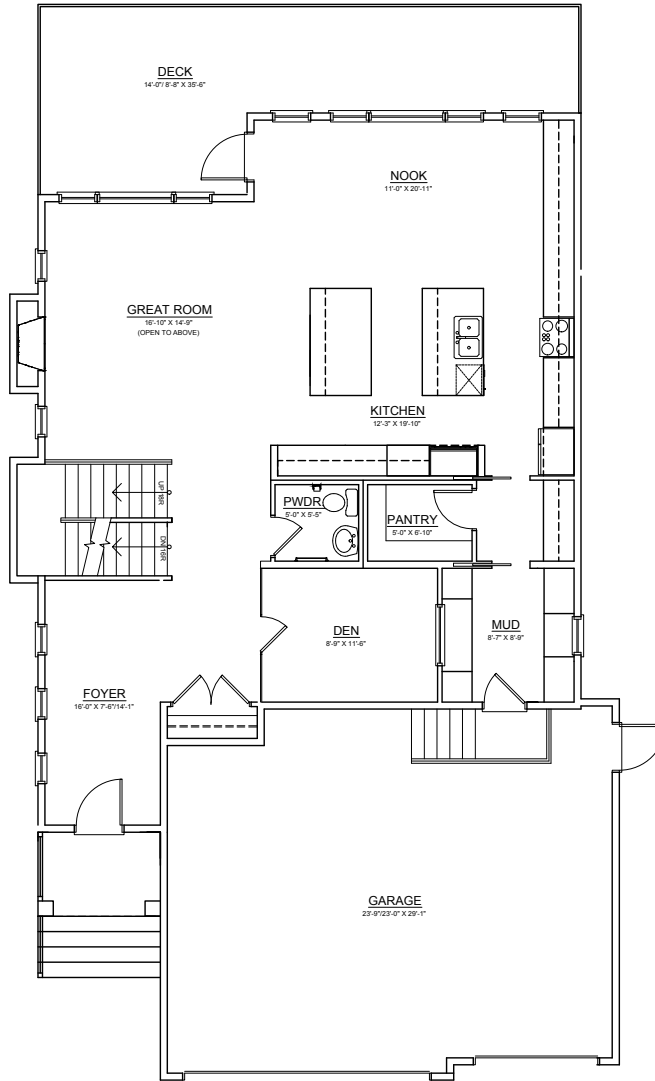
MAIN FLOOR ±1,464 SQ. FT.
