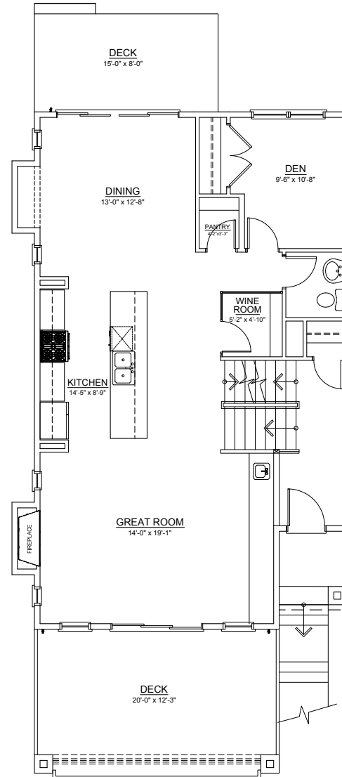
MAIN FLOOR ±1,072 SQ. FT.
