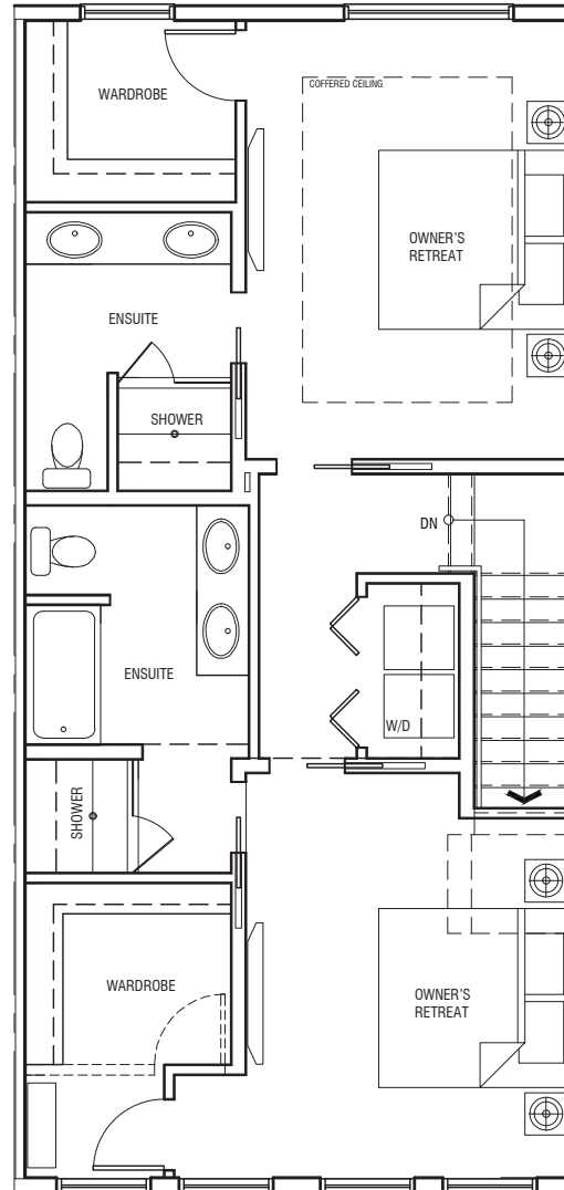
UPPER FLOOR ±800 SQ. FT.
