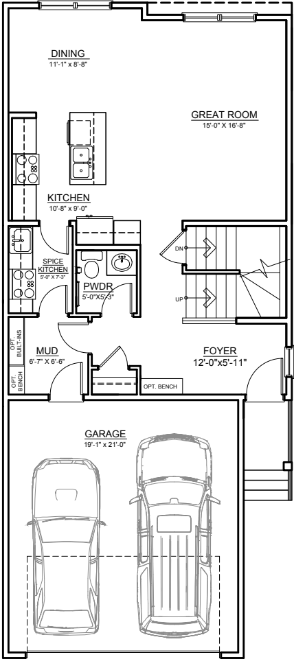
MAIN FLOOR OPTION 2 ±781 SQ.FT. | ADD SPICE KITCHEN
