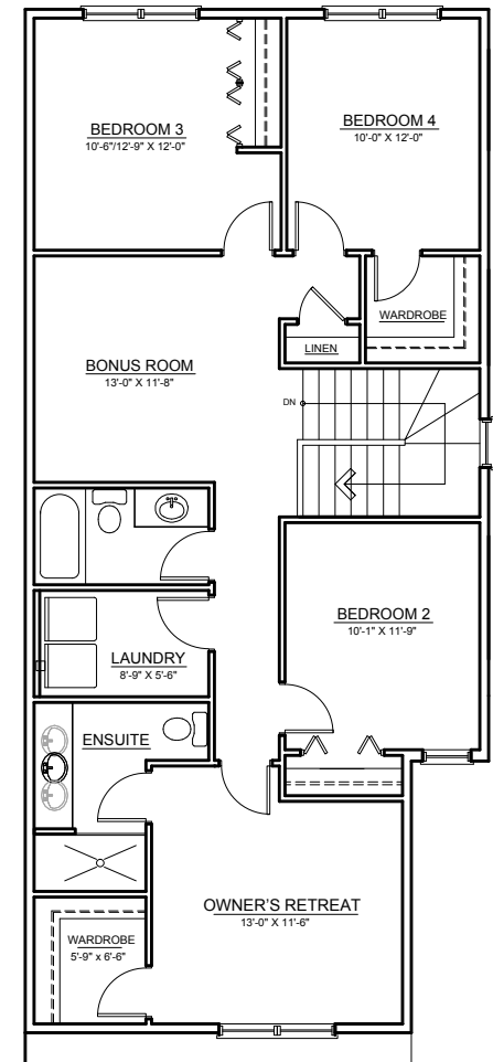
UPPER FLOOR OPTION 4 ±1,214 SQ.FT. | 4 BED + BONUS
