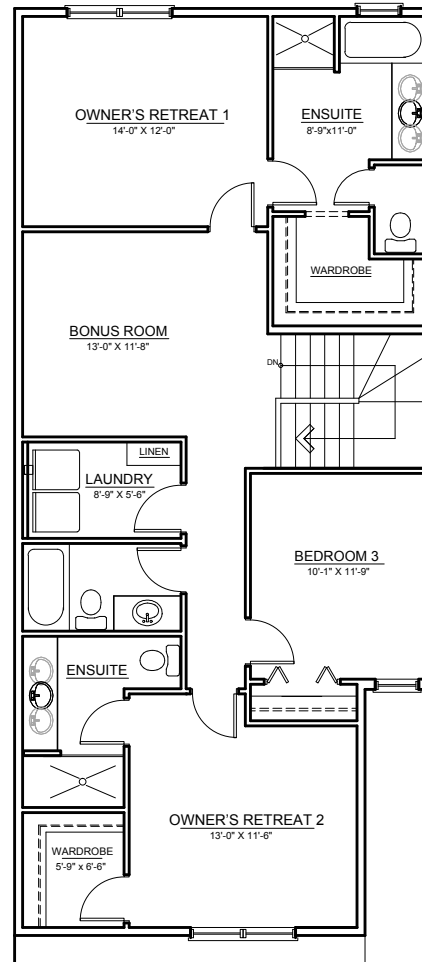
UPPER FLOOR OPTION 3 ±1,214 SQ.FT. | ALT. DOUBLE MASTER
