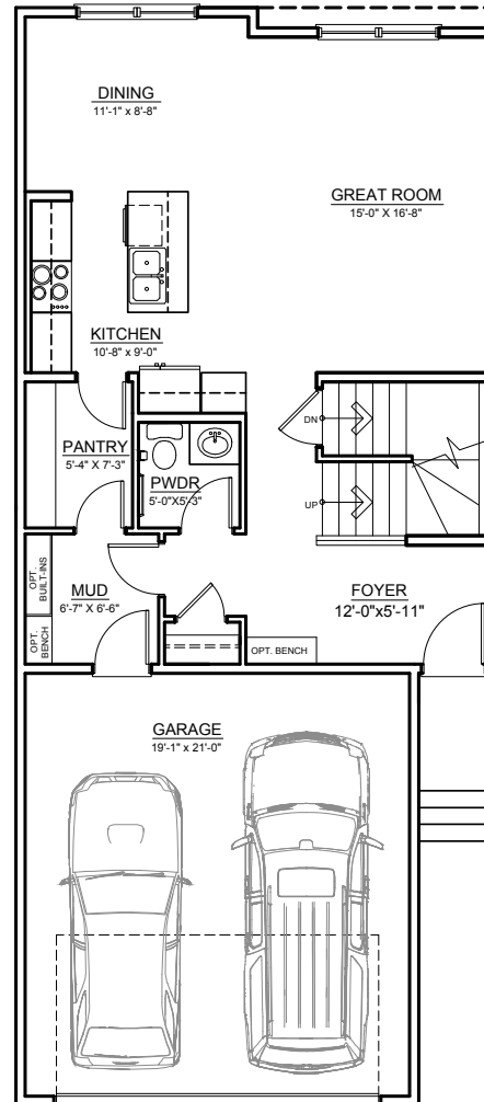
MAIN FLOOR OPTION I ± 781 SQ.FT.
