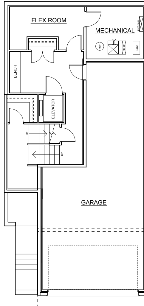
LOWER FLOOR ±363 SQ. FT.
