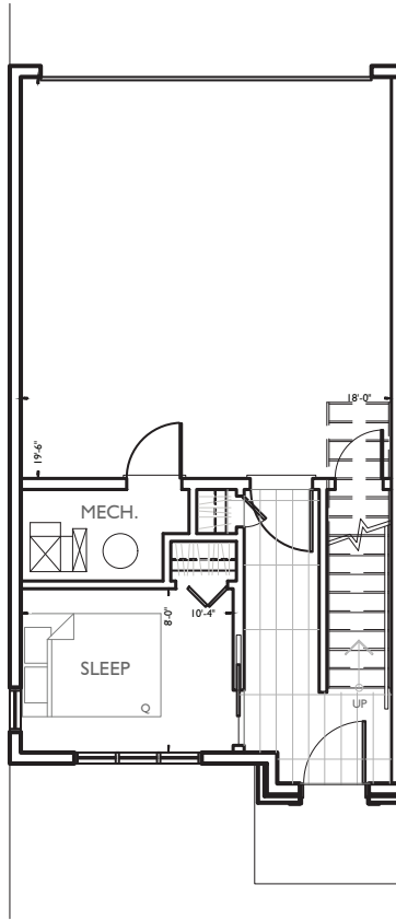
GROUND LEVEL 173 SQ. FT.
