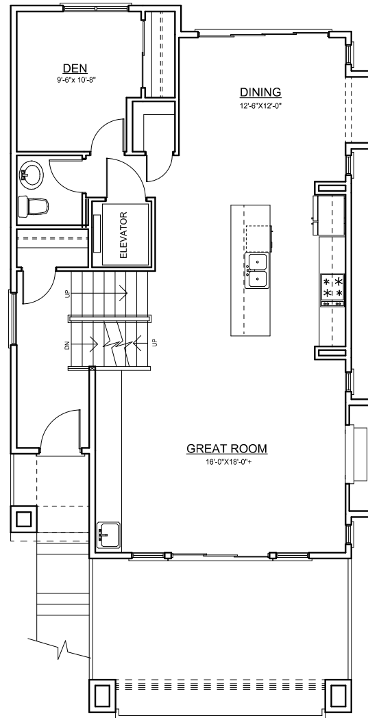
MAIN FLOOR ±1,052 SQ. FT.
