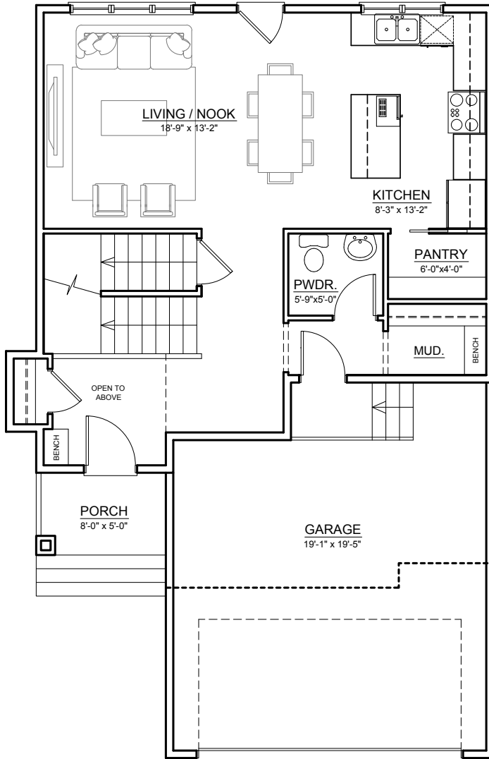
MAIN FLOOR ±722 SQ.FT.
