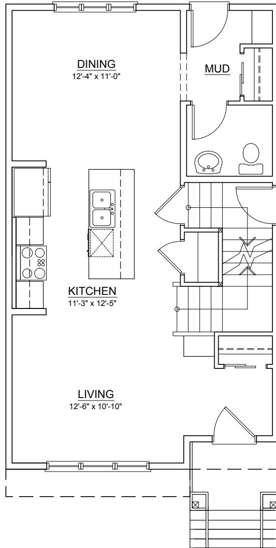
MAIN FLOOR ±667 SQ. FT.
