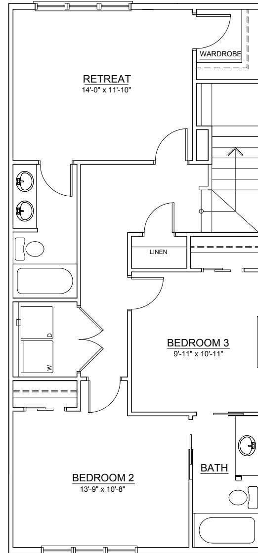
UPPER FLOOR ±860 SQ. FT.
