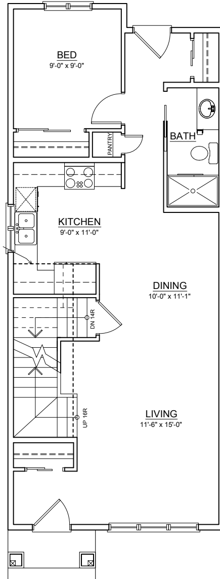
MAIN FLOOR ±776 SQ. FT.
