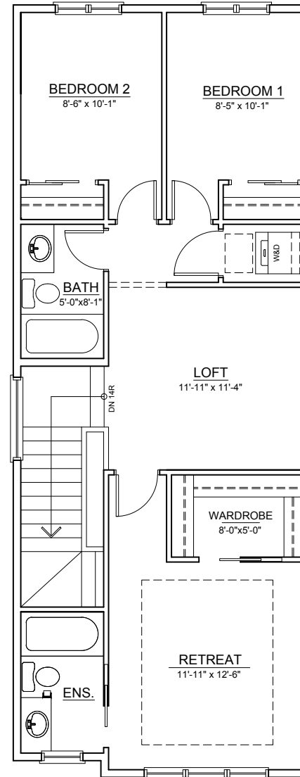
UPPER FLOOR ±831 SQ. FT.
