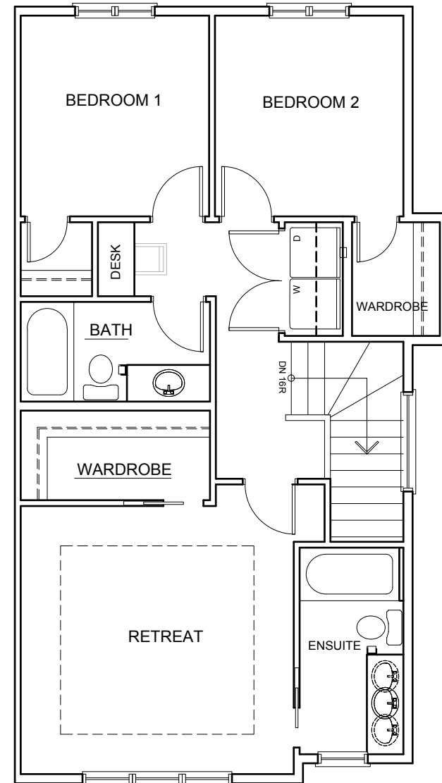
UPPER FLOOR \pm 747 SQ. FT.
