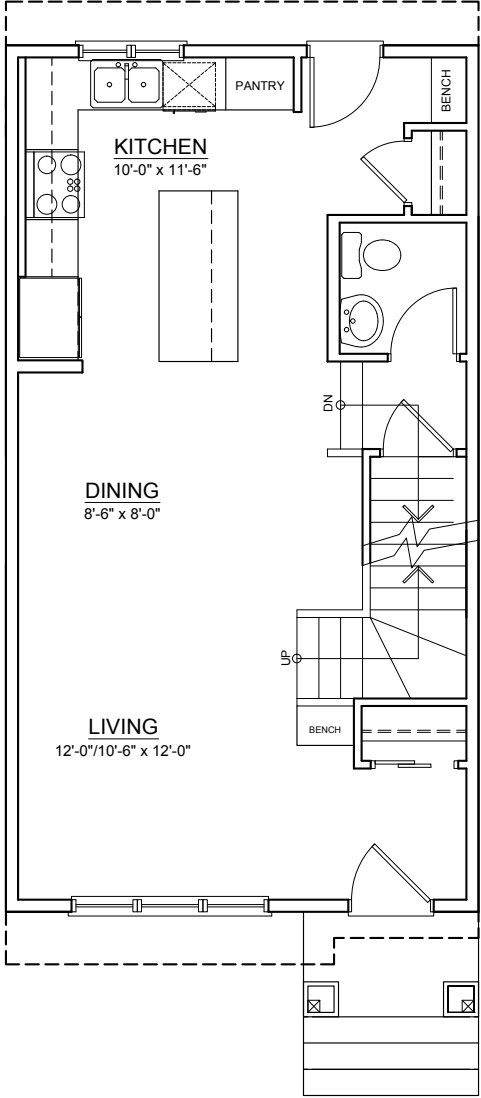
MAIN FLOOR ± 594 SQ. FT.
