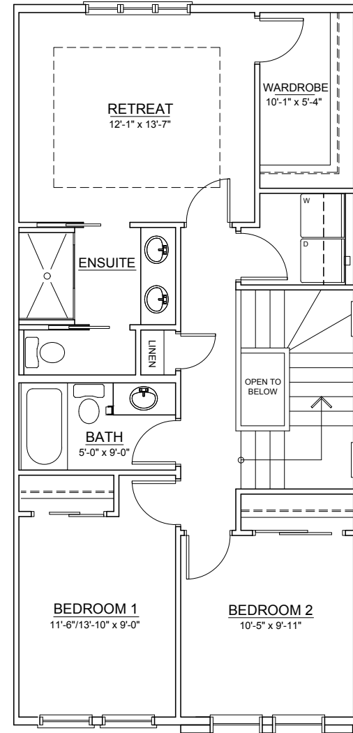
UPPER FLOOR OPTION I ±827 SQ. FT.
