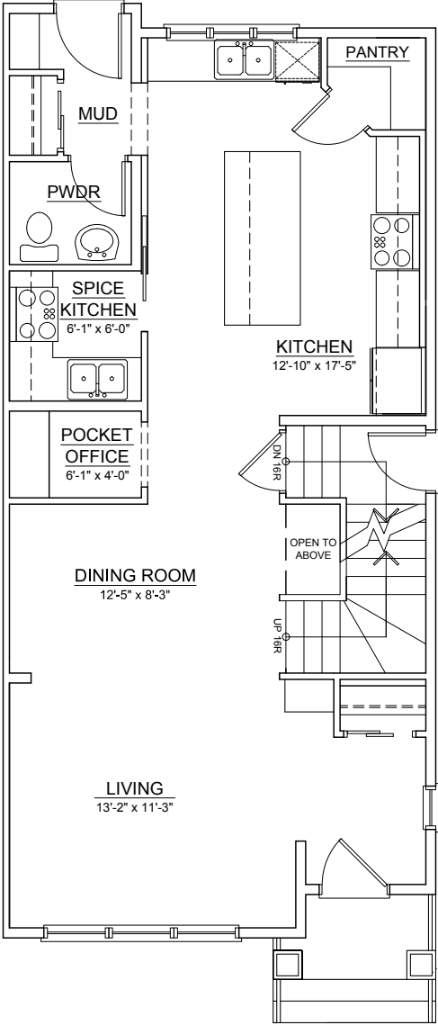
MAIN FLOOR OPTION 2 ±832 SQ. FT.
