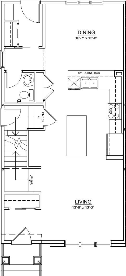
MAIN FLOOR ±780 SQ. FT.
