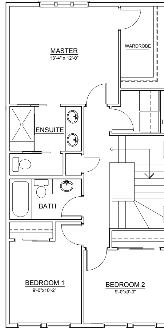
UPPER FLOOR ± 800 SQ. FT.
